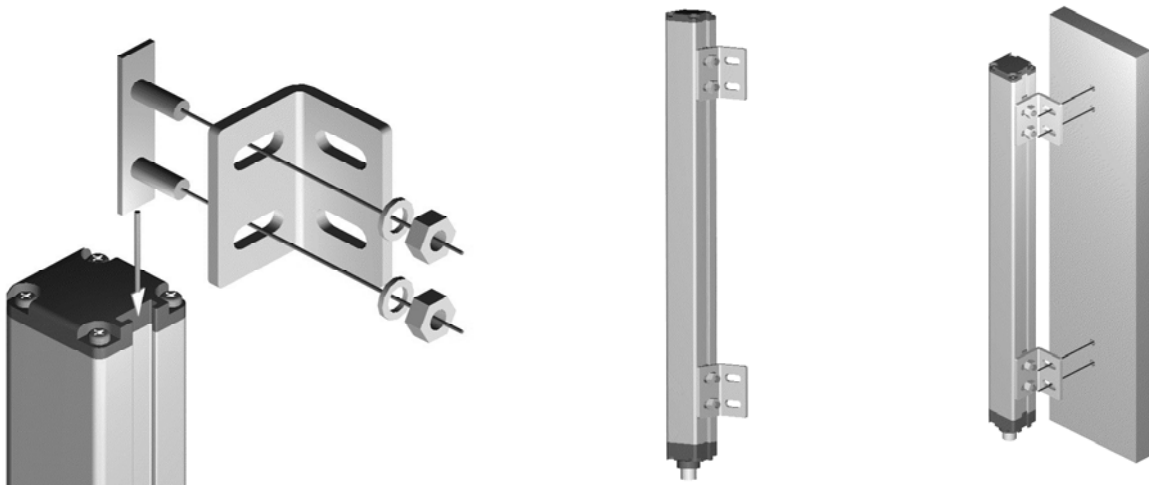
Figure 10 – Mechanical assembly
